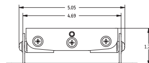
Front View: Add 3/4" (19 mm) for most interface brackets
